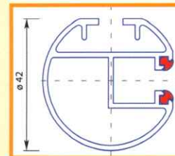
Rund-FS
