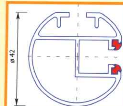
Rund-FS
